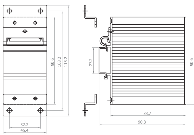
EHG2308 Front-panel view, Backboard rear view and Housing side view (including the optional mounting kit)
